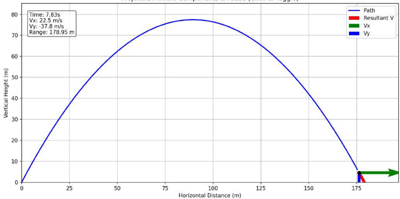
Projectile Motion: Components & Pause (Click to Toggle)
